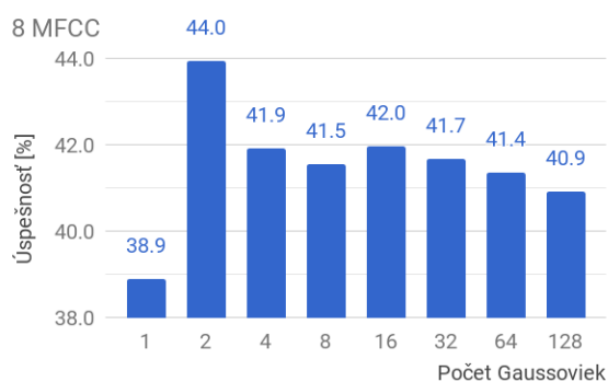
(a) 8 MFCC koeficientov
