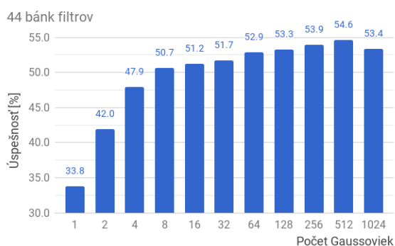
(g) 44 bank filterov
