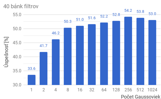
(f) 40 bank filterov
