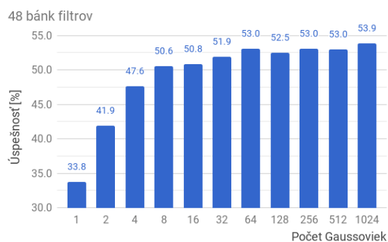
(h) 48 bank filterov
