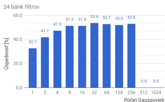
(b) 24 bank filterov
