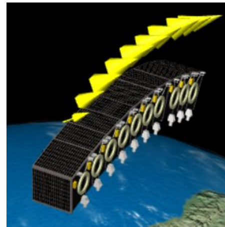
Particles directions
