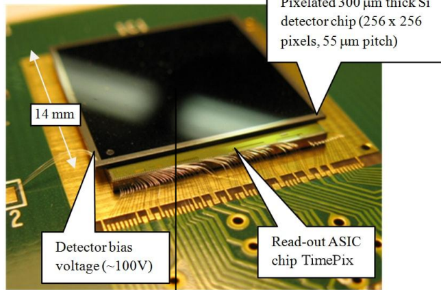
Timepix detector
