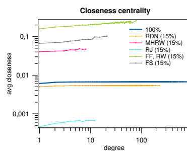
(h) Closeness centralita
