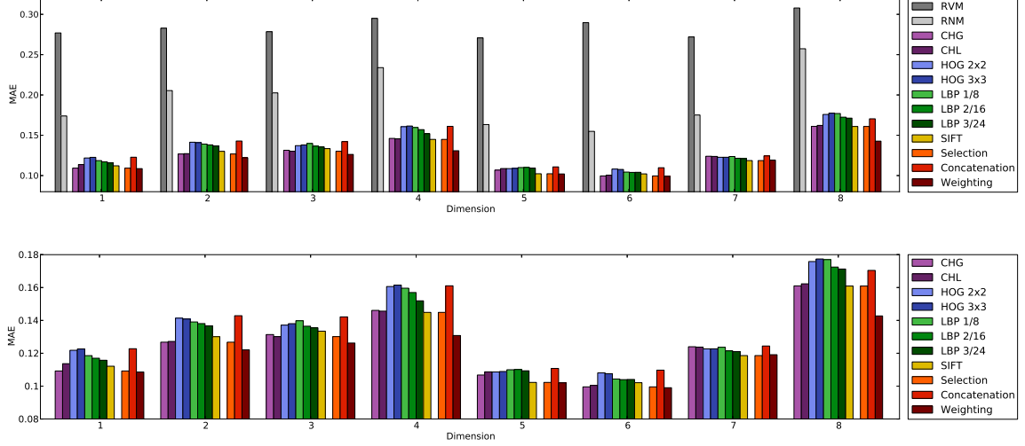
Figure 11.1: Per-dimension MAE for the Food-1000 dataset. The top image shows the error values in context of the RVM and RNM predictions while the bottom one zooms to the differences among the evaluated methods. The best single-feature methods were CHG, CHL and SIFT, the total best values were obtained with feature weighting while feature concatenation failed to work.
