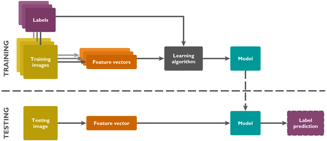
Figure 5.5: Supervised learning from images. The system aims to learn the relation between feature vectors and data labels. A prediction is an estimated label value.
